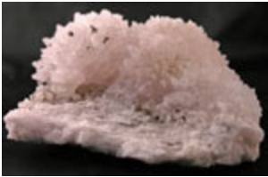
Mangano-calcite Broken Hill, New South Wales, Australia
