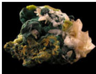
Malachite, Cerussite
